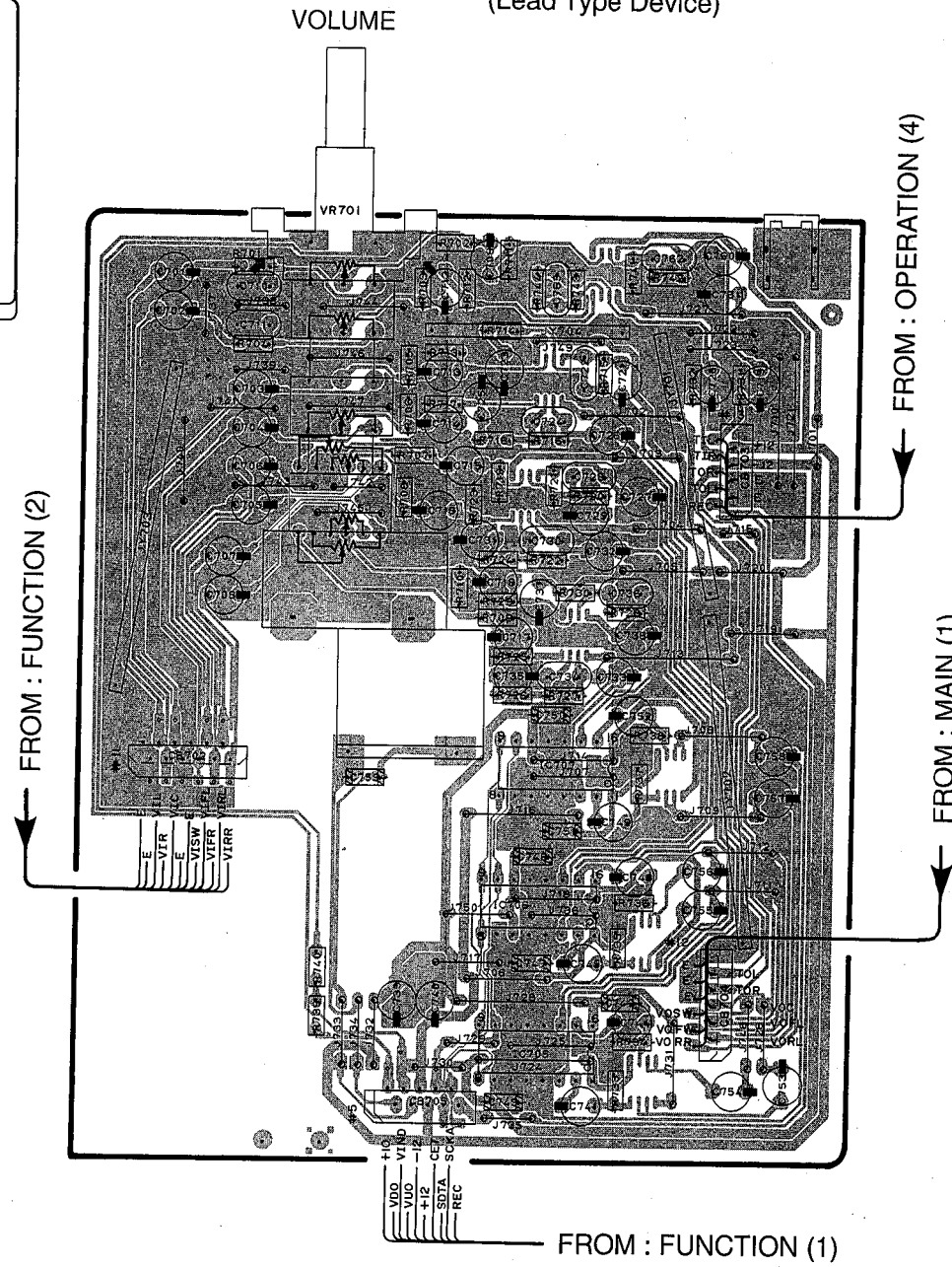
P. C. B. VIDEO ( 3 ) (Lead Type Device)
