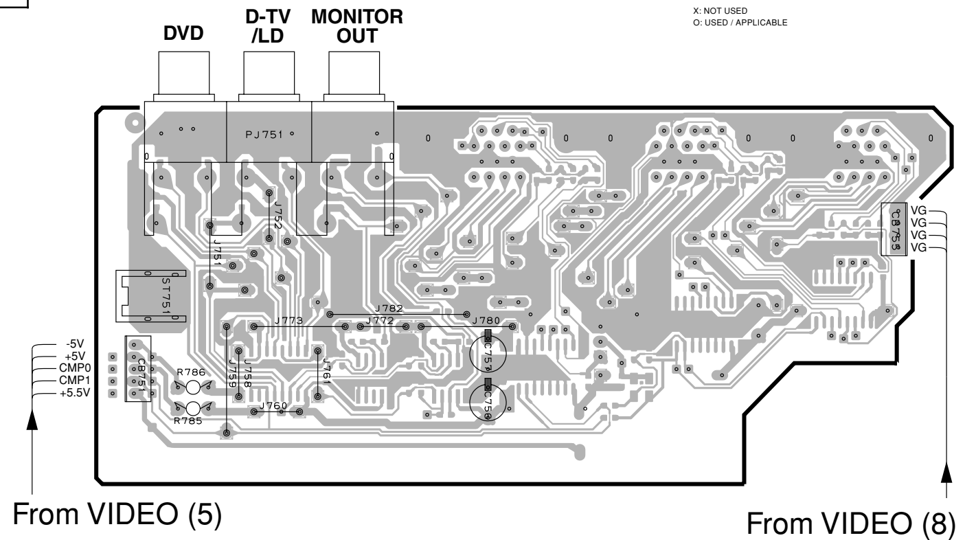
VIDEO (4) P. C. B. (Surface Mount Device)
