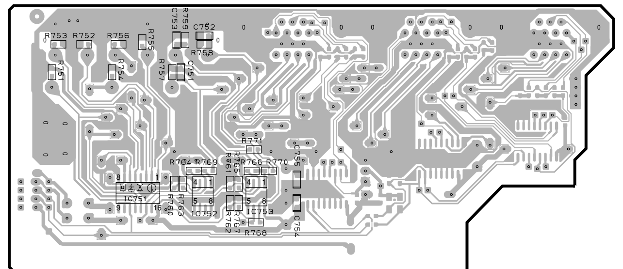
VIDEO (4) P. C. B. (Surface Mount Device)
