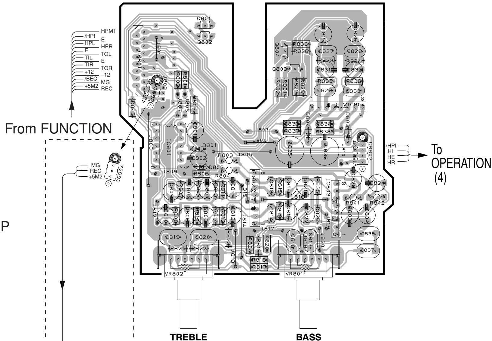
OPERATION (5) P. C. B. (Lead Type Device)
