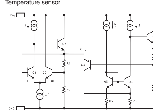
IC238: LM61CIZ Temperature sensor
