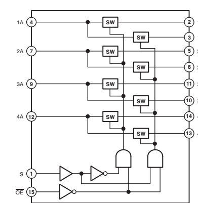
IC907: SN74CB3Q3257PWR Low voltage high-bandwidth bus switch
