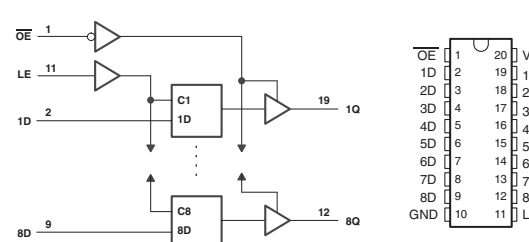
IC204-206: SN74LV573APWR Octal transparent D-type latches with 3-state outputs
