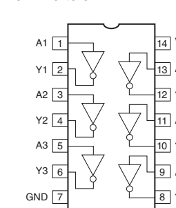
IC305: SN74LVU04APWR Hex inverters
