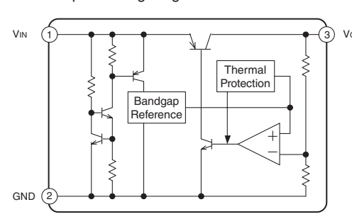
IC905: NJM2885DL1-33 Low dropout voltage regulator
