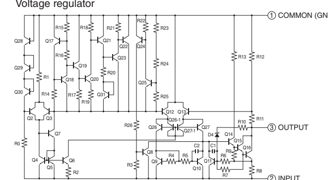
IC237: KIA7912PI Voltage regulator
