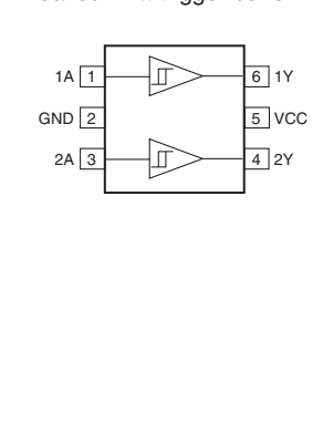
IC908: SN74LVC2G17DCKR Dual schmitt-trigger buffer
