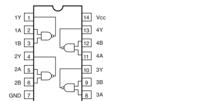
IC203: SN74AHC02PWR Quadruple 2-input positive-NOR gates
