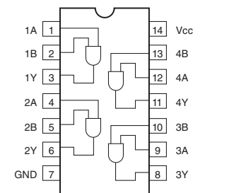
IC505: SN74LV08APWR Quaduple 2-input positive-AND gate
