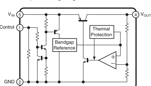
IC902: NJM2867F3-05 Low dropout voltage regulator
