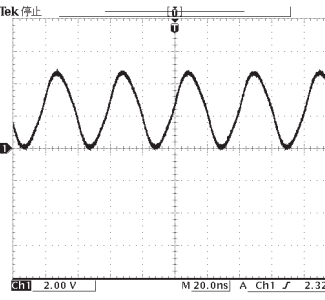
POINT (B) XL301 (Pin 6 of IC301)
