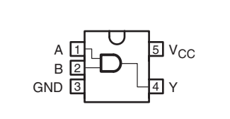
IC906: SN74LVC1G08DCKR Single 2-input positive-AND gate
