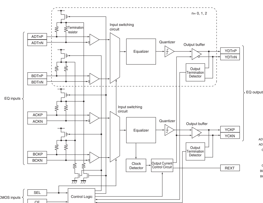
IC903: CXB1442AR-T4 Cable equalizer with 2-system switching function
