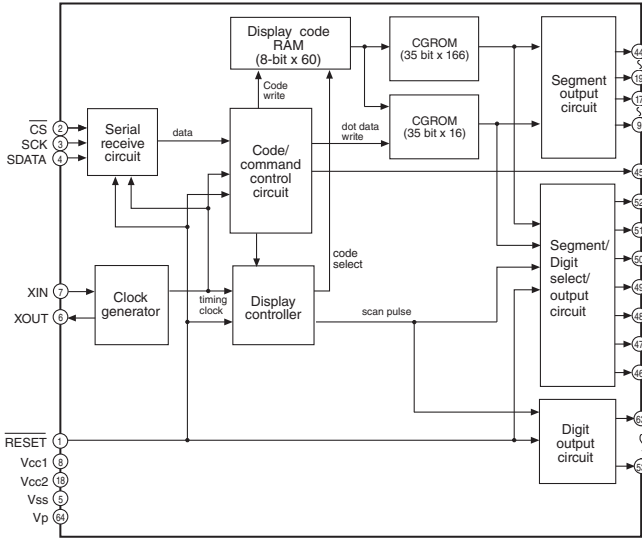
IC201: M66003-0131FP-R (OPERATION P.C.B.) 18 digit 5x7 segment VFD controller/driver
