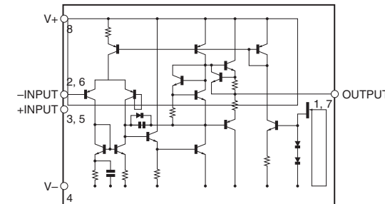
IC23, 24, 25, 27: NUM4565M (TE1) Dual operational amplifier
