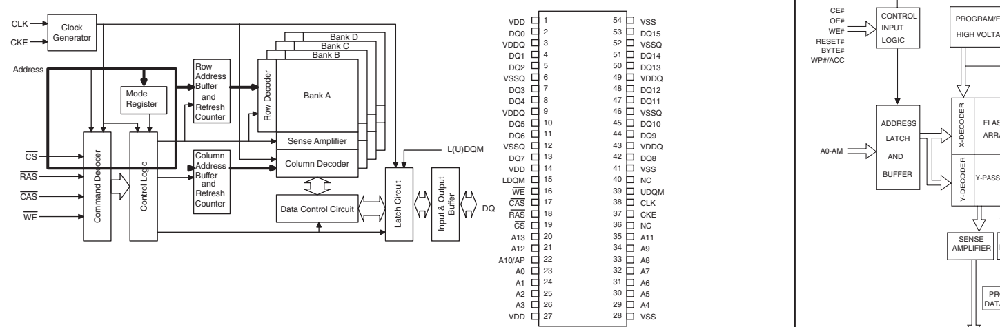
IC242: M12L64164A-5TG 1M x 16-bit x 4 banks synchronous DRAM
