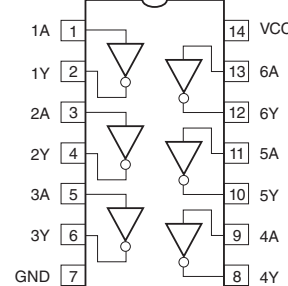
IC22: TC74VHC04FT Hex inverters
