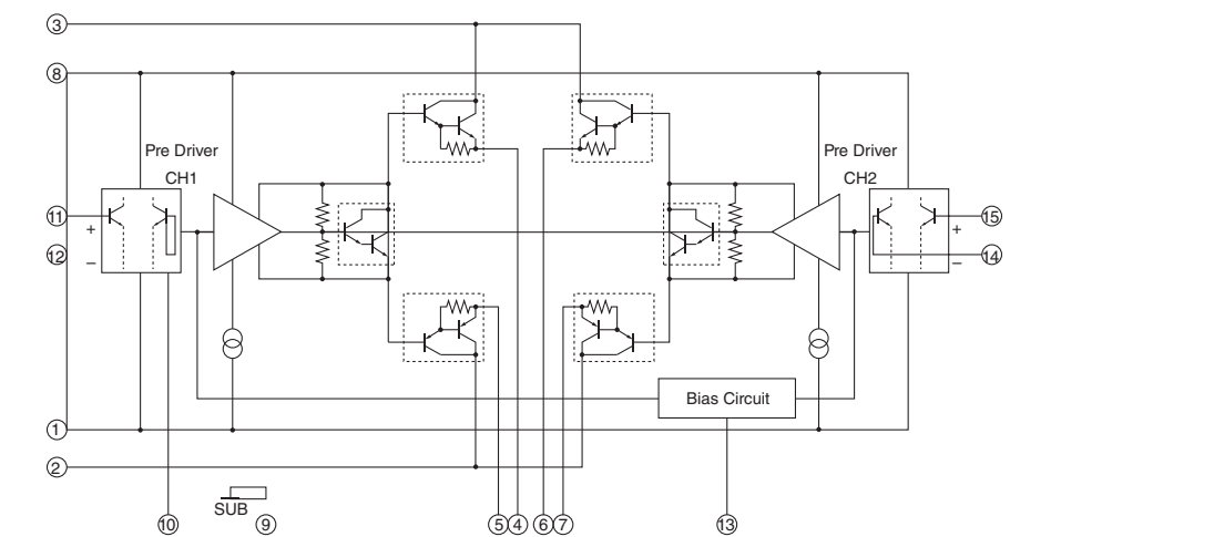
IC2: STK433-130Y-E 2-channel AF power amplifier, stand-by circuit built-in
