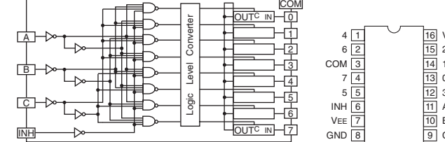
IC42: TC74HC4051AFEL 8-channel analog multiplexer/demultiplexer
