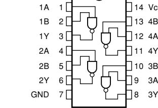
IC805: TC74HC00AF IC808: TC74HCU04AF Quad 2-Input Nand Gate
