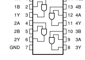
IC806: TC74VHCT08AF Quad 2-Input And Gate
