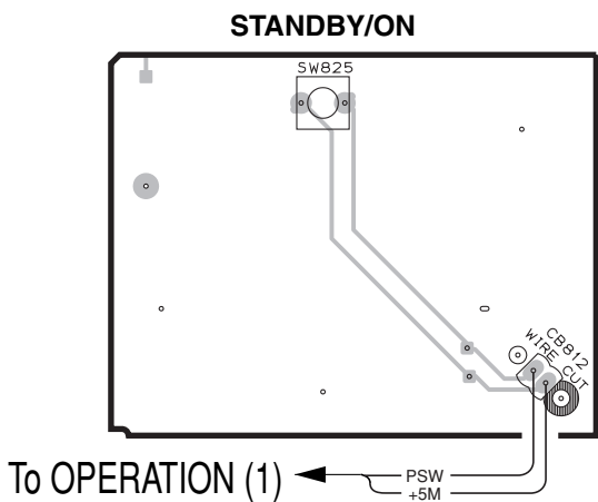
OPERATION (7) P. C. B.
