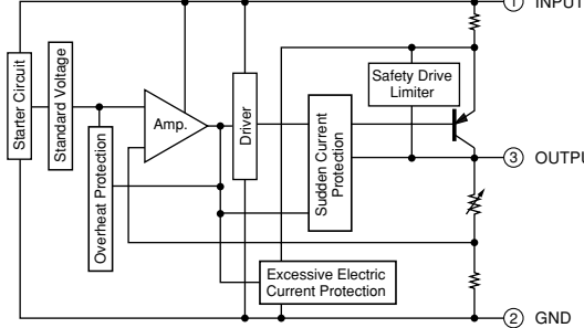
IC804: μPC29M33T-E1 Voltage Regulator
