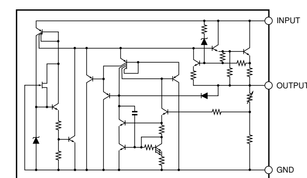
IC903: NJM78L05A-T3 Voltage Regulator
