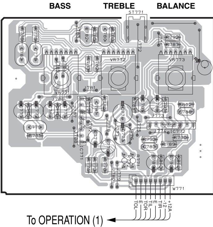
OPERATION (7) P. C. B.
