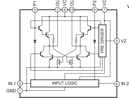
IC734: LB1641 Motor Driver
