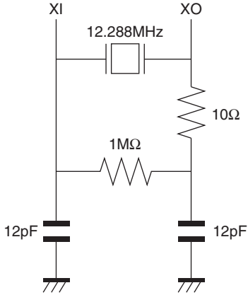
Note 2) Example of crystal oscillator connection circuit
