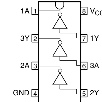
IC904: SN74LVC3G04DCTR Triple inverter gate
