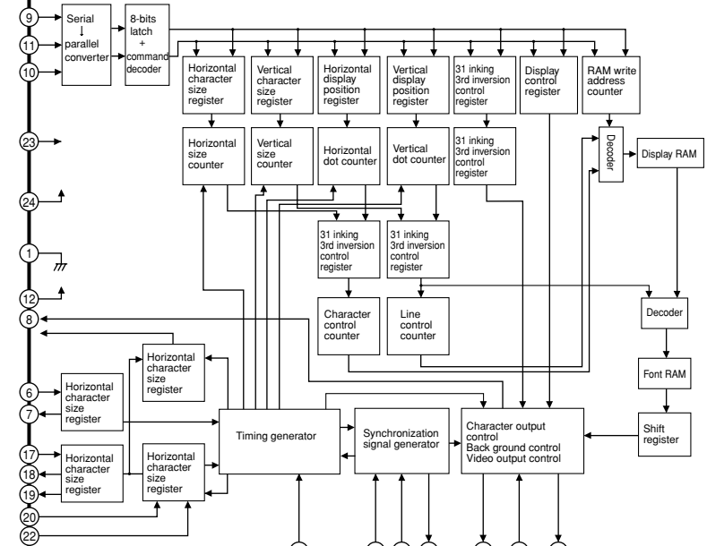
IC342: LC74782JM-8A16-TLM The on-screen display controller LSI
