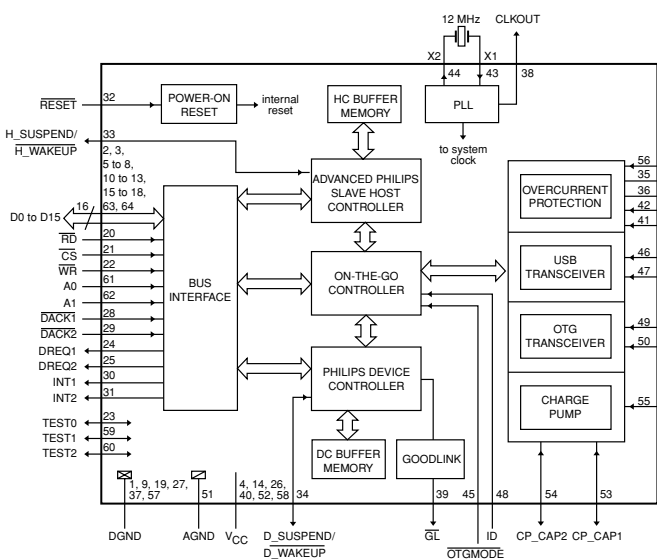
IC601: ISP1362BD Single-chip universal serial bus on-the-go controller
