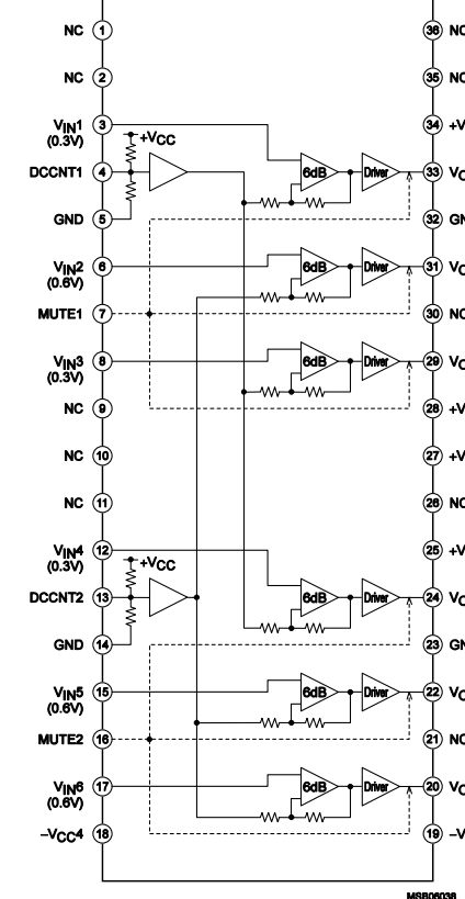
IC344: LA73050-TLM-E 6-channel 75-ohm video driver
