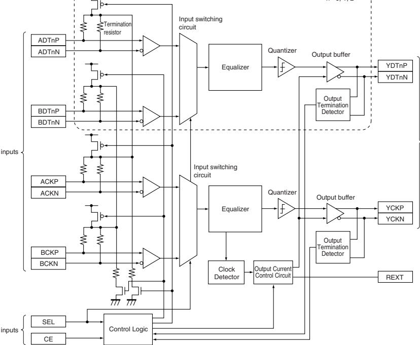
IC903: CXB1442AR-T4 Cable equalizer with 2-system switching function
