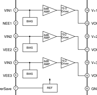
IC321: NJM2581M Video amplifier
