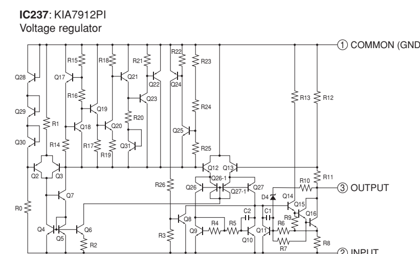
IC237: KIA7912PI Voltage regulator
