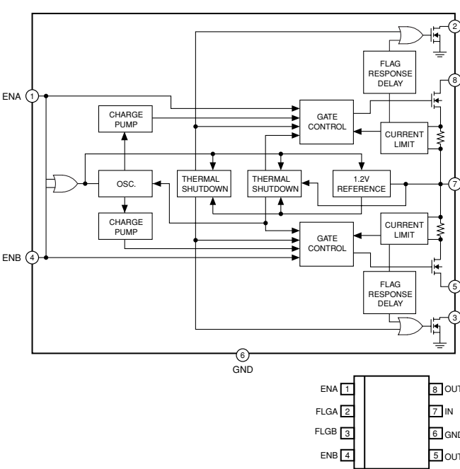
IC602: MIC2026-2BM Dual-channel power distribution switch
