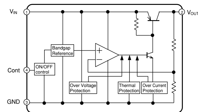
IC232: NJM2388F33 Low dropout voltage regulator with ON/OFF control
