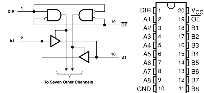
IC404: SN74AHC245PWR Octal bus transceivers with 3-state outputs
