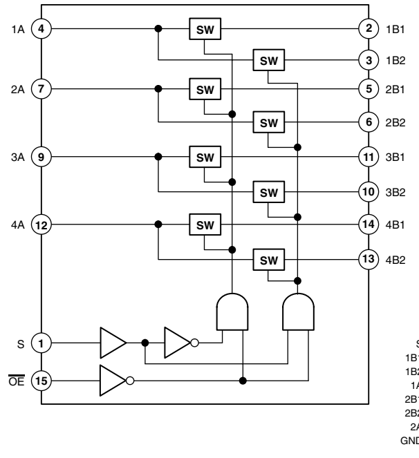
IC905: SN74CB3Q3257PWR Low voltage high-bandwidth bus switch
