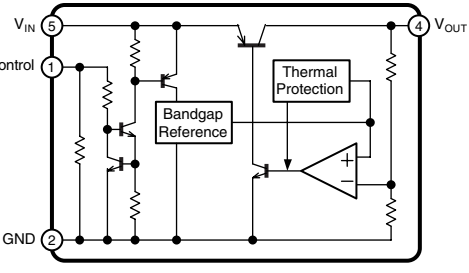
IC902: NJM2867F3-05 Low dropout voltage regulator
