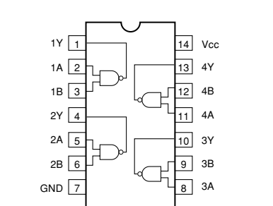
IC203: SN74AHC02PWR Quadruple 2-input positive-NOR gate
