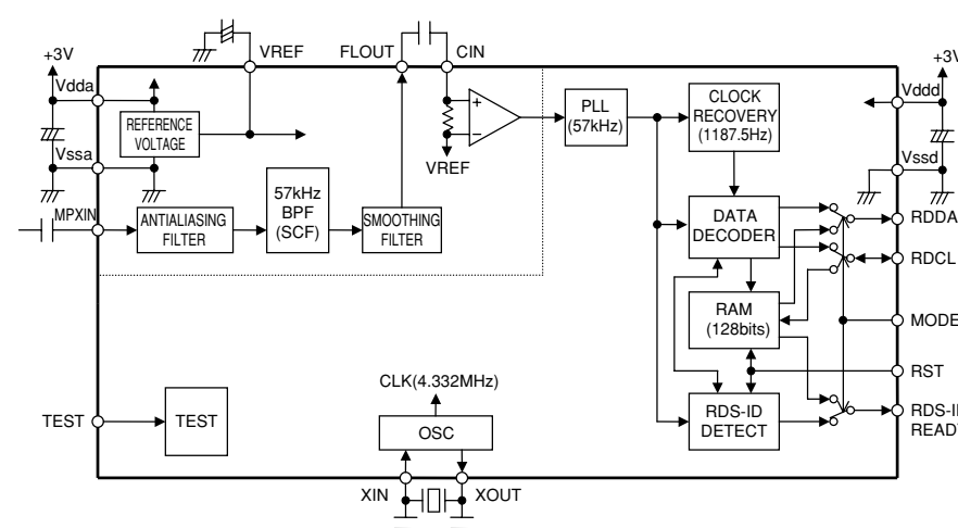
IC168: LC72725KM RDS signal demodulation IC
