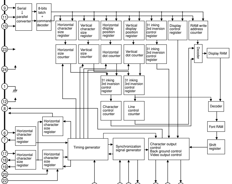
IC342: LC7482JM-8A16-TLM The on-screen display controller LSI
