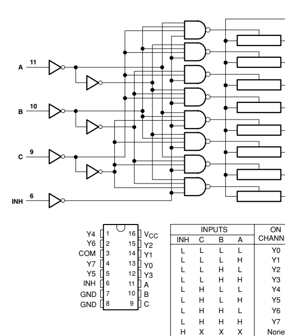
IC402, 403: SN74LV4051APWR 8-channel analog multiplexers/demultiplexers
