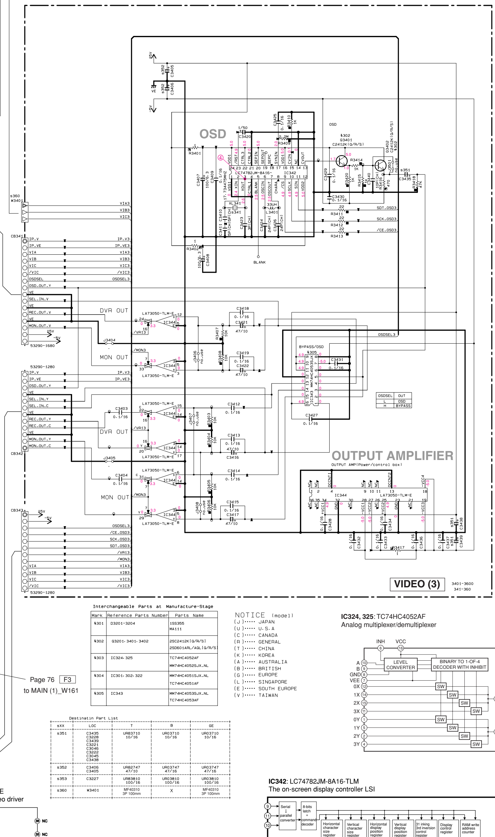
IC321: NJM2581M Video amplifier
