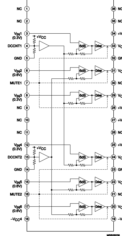
IC344: LA73050-TLM-E 6-channel 75-ohm video driver
