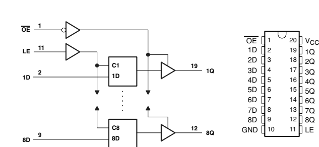
IC204-207: SN74LV573APWR Octal 3-state D-latches with 3-state output:
