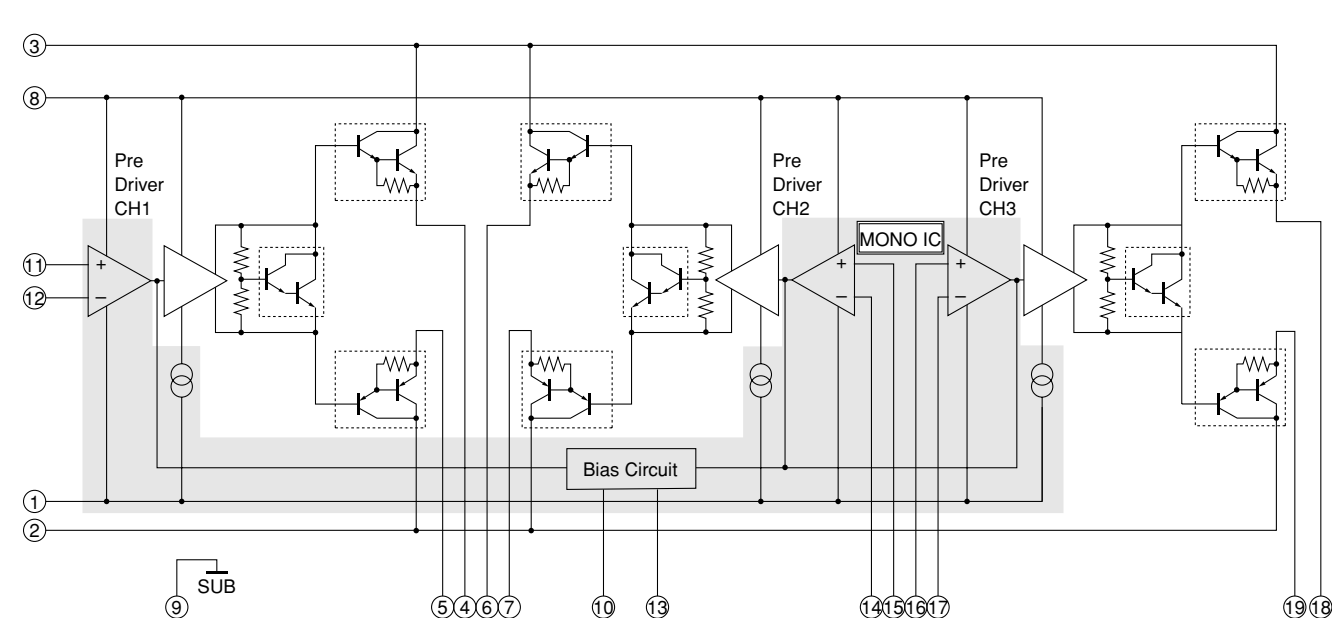
IC101: STK433-330-E 3-channel AF power amplifier, stand-by circuit built-in
