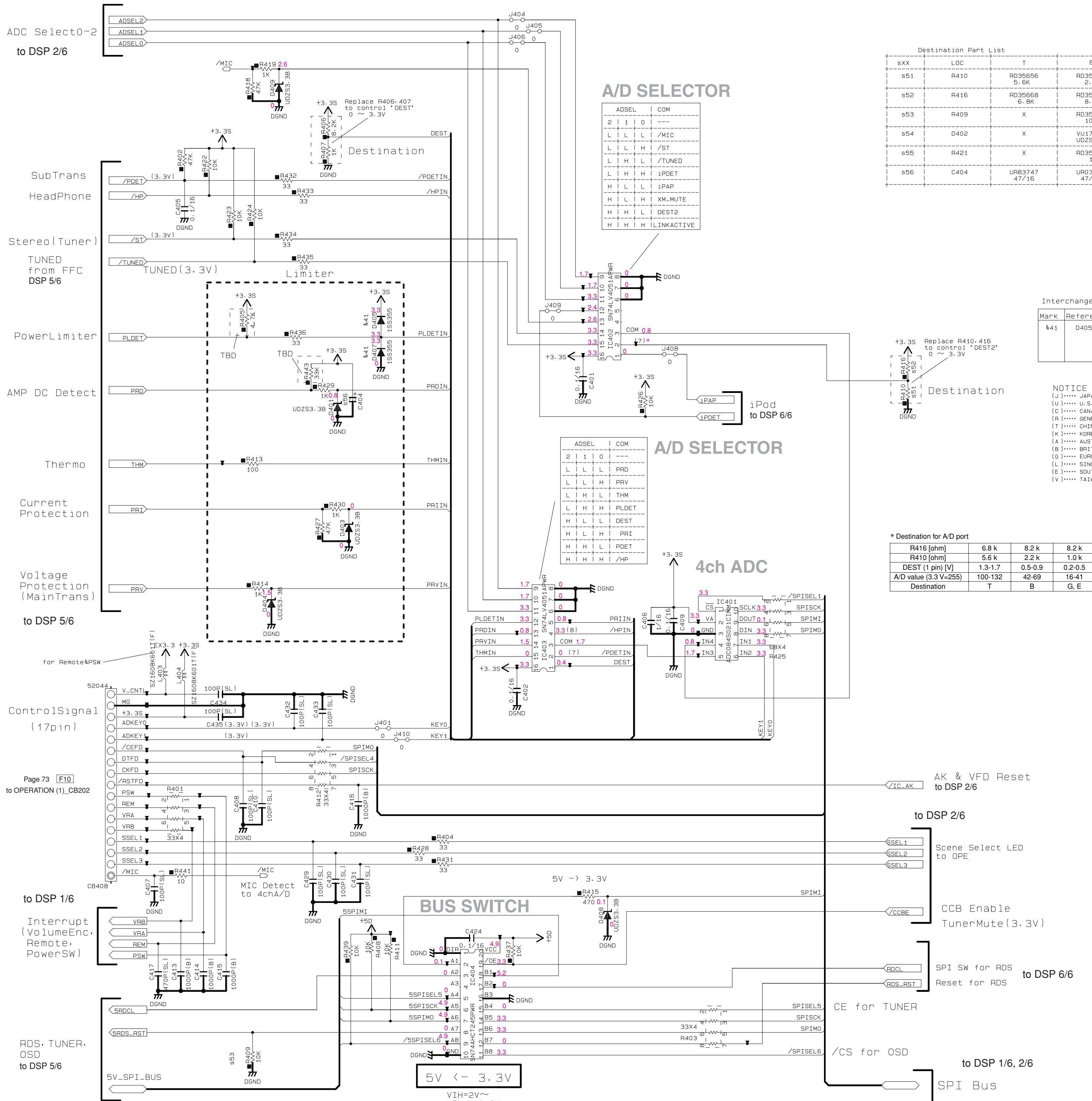
IC402, 403: SN74LV4051APWR 8-channel analog multiplexers/demultiplexers
