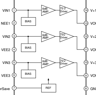
IC321: NJM2581M Video amplifier
