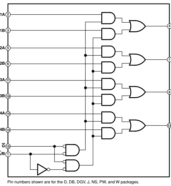
IC302: SN74LV157APWR Quadruple 2-line to 1-line data selectors/multiplexers
