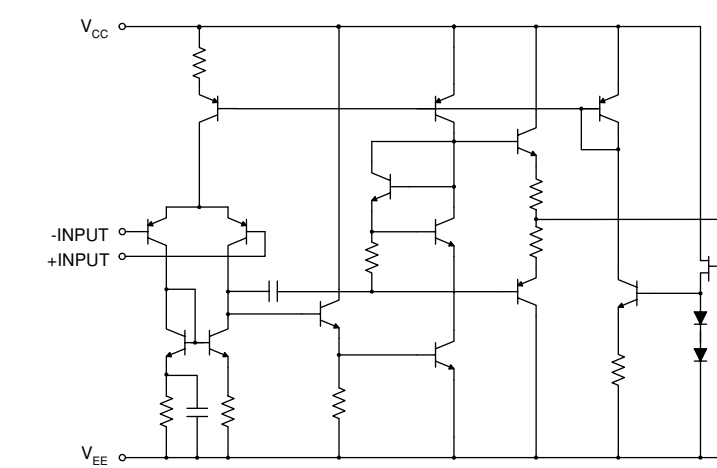
IC162-164, 169: AZ4580MTR-E1 Dual low noise operational amplifiers
