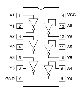
IC305: SN74LVU04APWR Hex inverters
