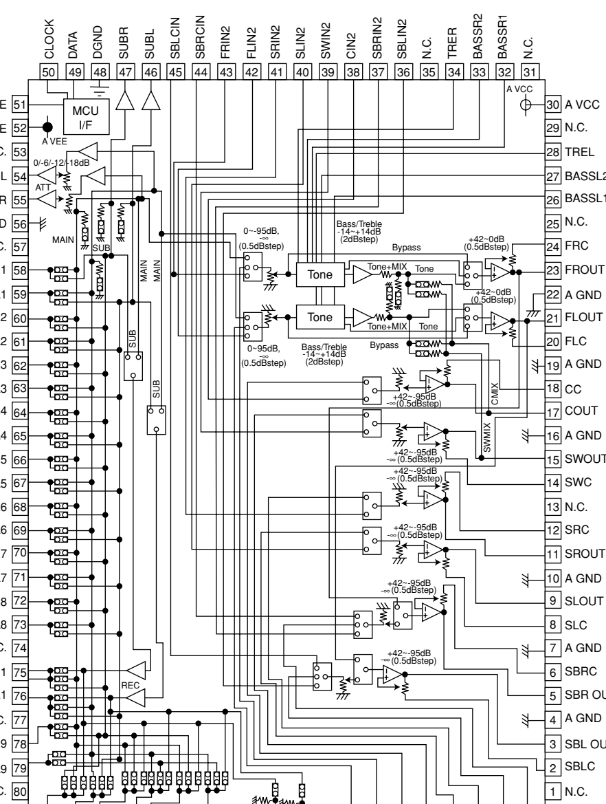
IC161: R2A15215FP 8-channel electronic volume with 11 input selector and tone control
