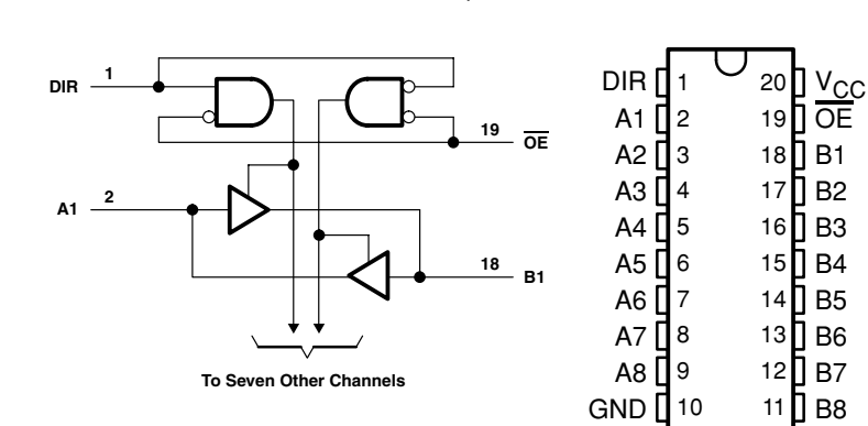
IC404: SN74AHC245PWR Octal bus transceivers with 3-state outputs
