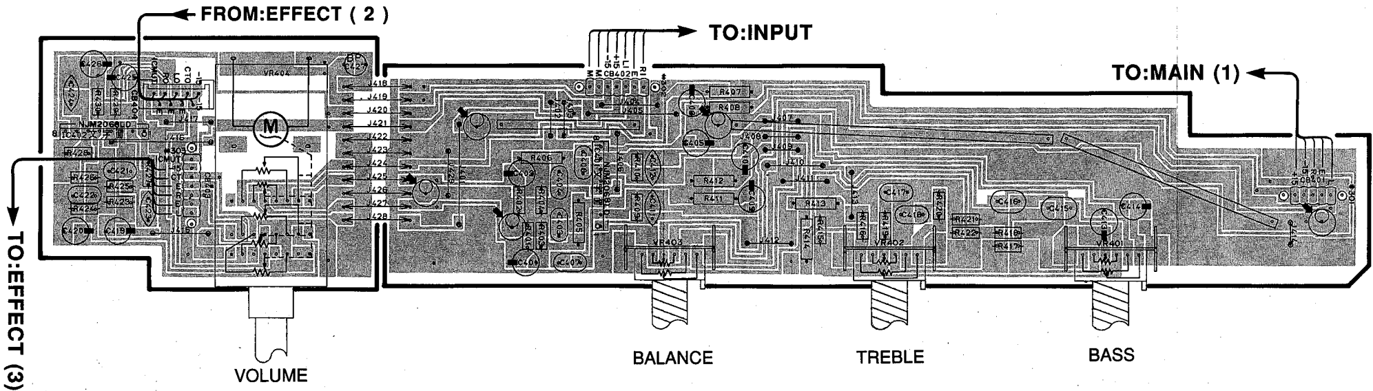
P.C.B. OPERATION ( 2 )
