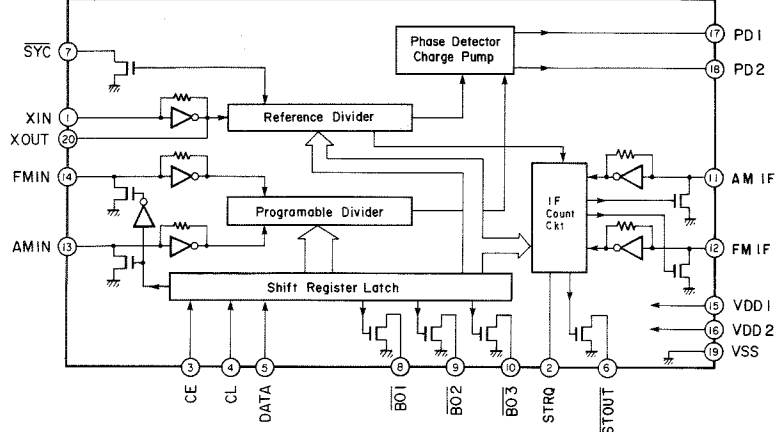
IC2 : LM7000N PLL Controller
