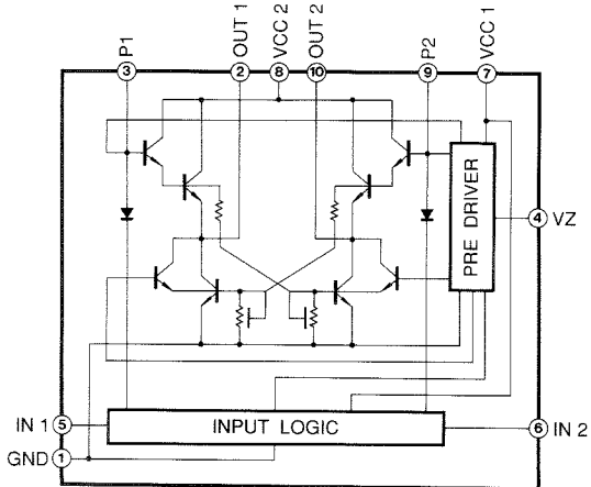
IC505 : LB1641 Motor Driver
