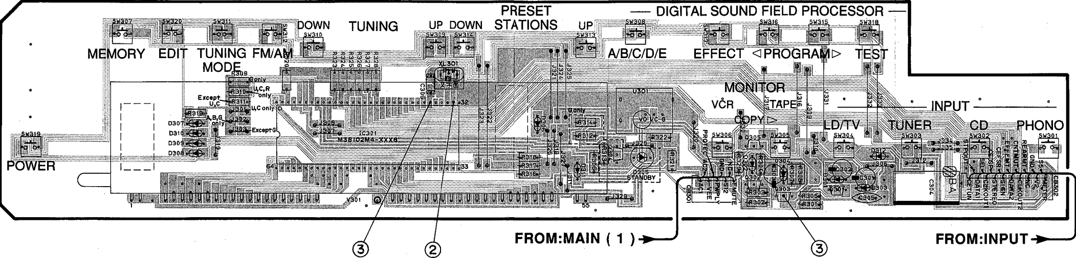
P.C.B. OPERATION ( 1 )
