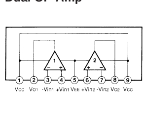
IC105, 106, 112, 113 : \mu PC4570HA Dual OP-Amp
