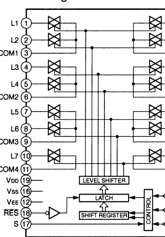
IC102 : LC78213 Analog Function Switch
