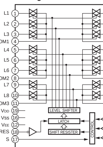
IC103 : LC78212 Analog Function Switch
