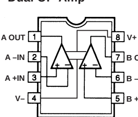
IC401-403 : \mu PC4570C Dual OP-Amp
