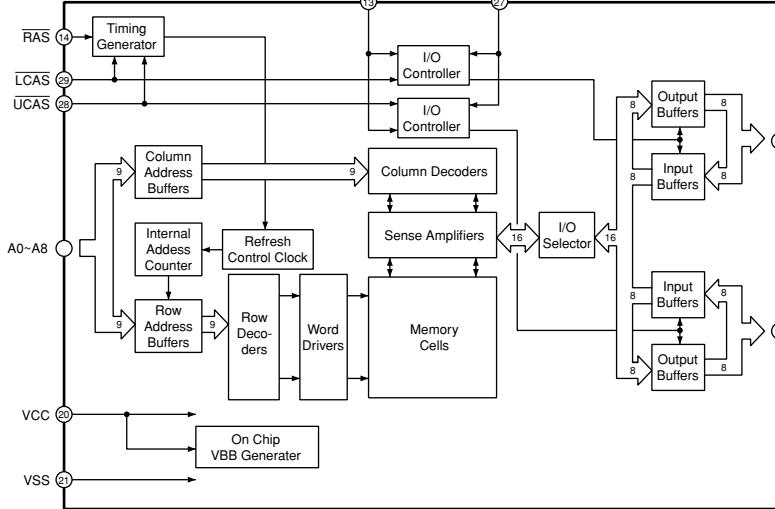
IC802: MSM514260C-60JS 4Mbit DRAM
