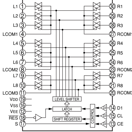
IC734: LB1641 Motor Driver
