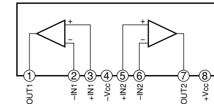
IC731~733: \mu PC4570C Dual OP-Amp
