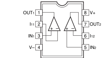
IC731~733: \mu PC4570C Dual OP-Amp
