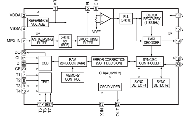
IC445: LC72722 RDS Decoder
