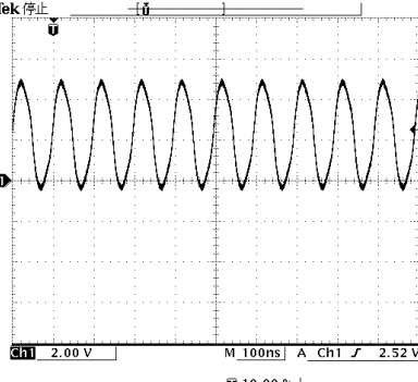
Point ③ Pin 15 of IC571
