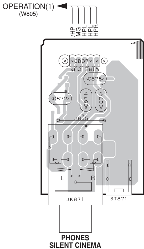
OPERATION (3) P.C.B. (Side A)
