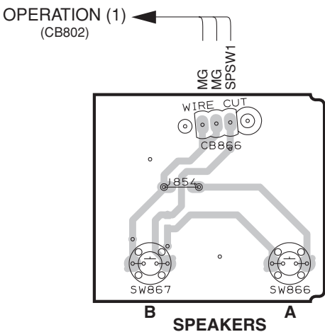
OPERATION (5) P.C.B. (Side A)
