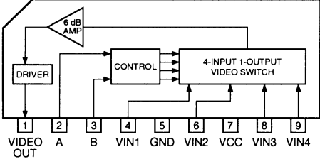
IC301~303 : LA7956 Video Switch
