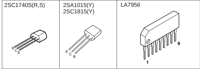
PIN CONNECTION DIAGRAM OF TRANSISTORS AND IC's.
