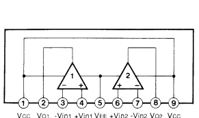
IC105, 106, 112, 113 : \mu PC4570HA Dual OP-Amp
