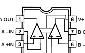
IC401-403 : \mu PC4570C Dual OP-Amp
