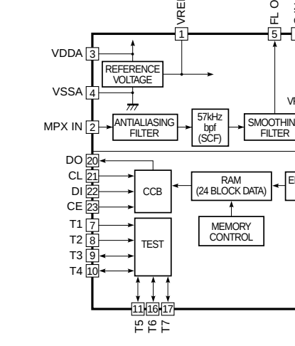
IC308 : LC72722 RDS Signal Processor
