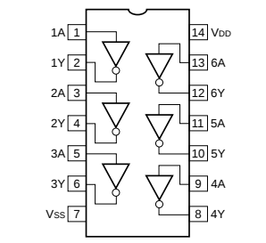
IC585 : TC74HCU04AP Hex Inverters
