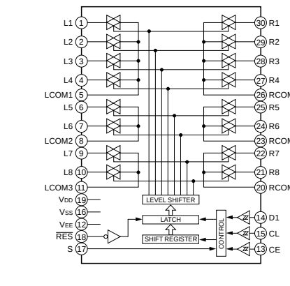
IC301, 303 : LC78211 Analog Function Switch
