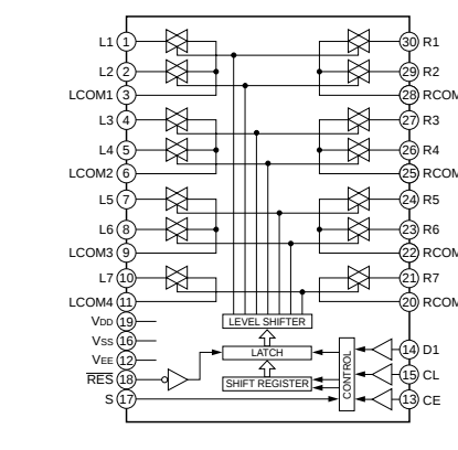
IC302, 304 : LC78213 Analog Function Switch
