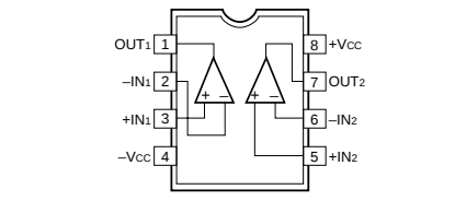
IC311-317, 319, 320 : μPC4570G2 Dual OP-Amp
