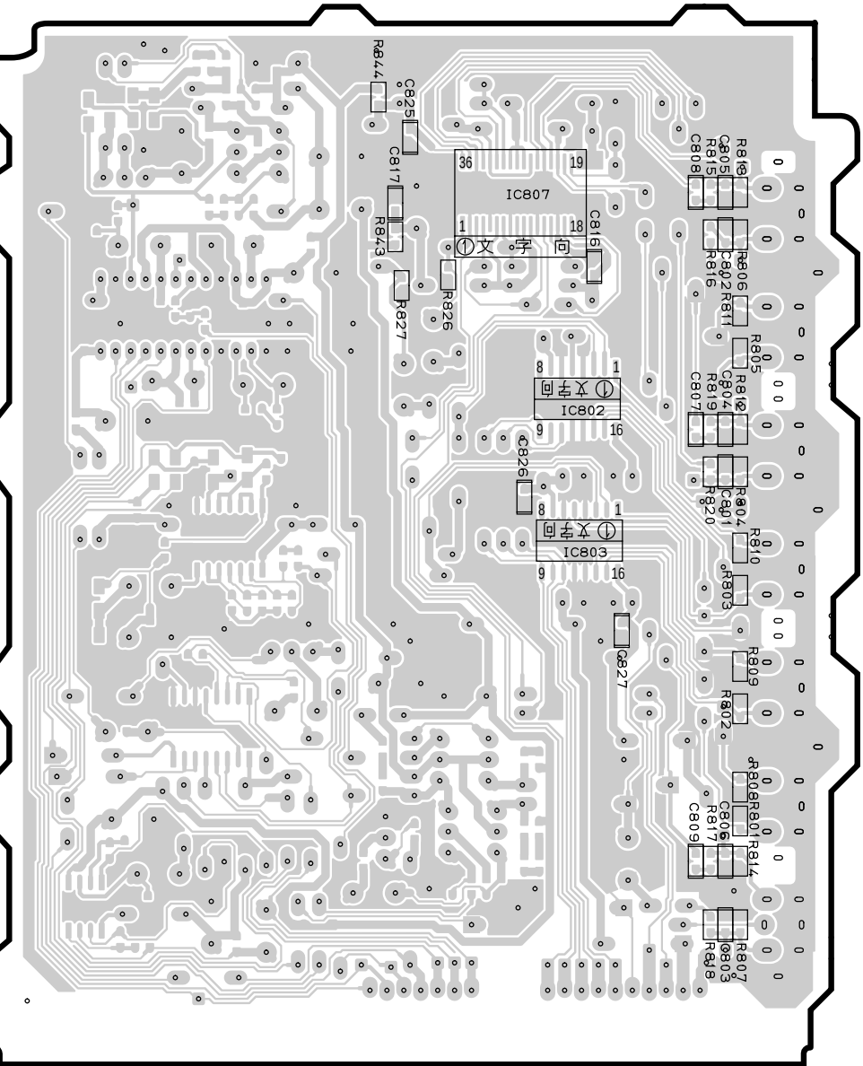
FUNCTION (5) P. C. B. (Surface Mount Device)
