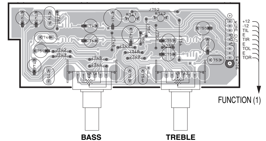
OPERATION (5) P. C. B. (Lead Type Device)
