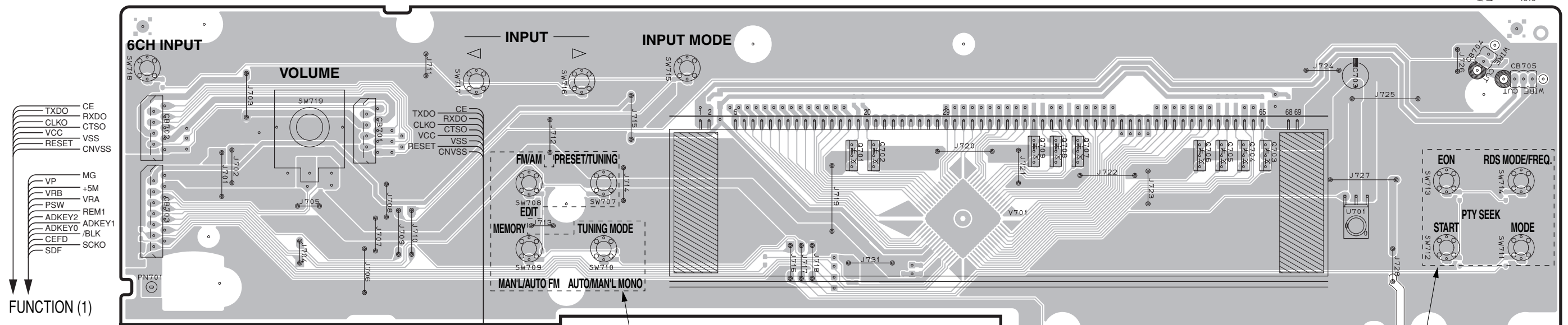
OPERATION (1) P. C. B. (Lead Type Device)
