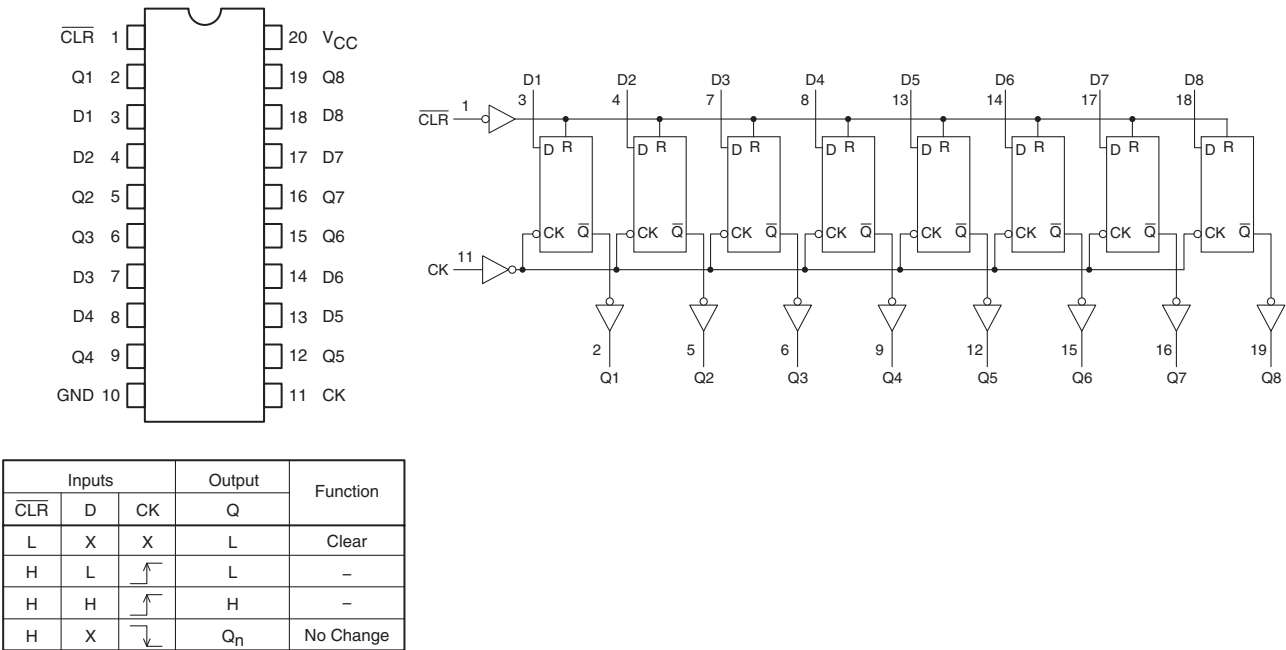
IC79, 81: TC74VHC273FT (EL,K) (DIGITAL (1) P.C.B.) Octal D-type flip-flop with clear
