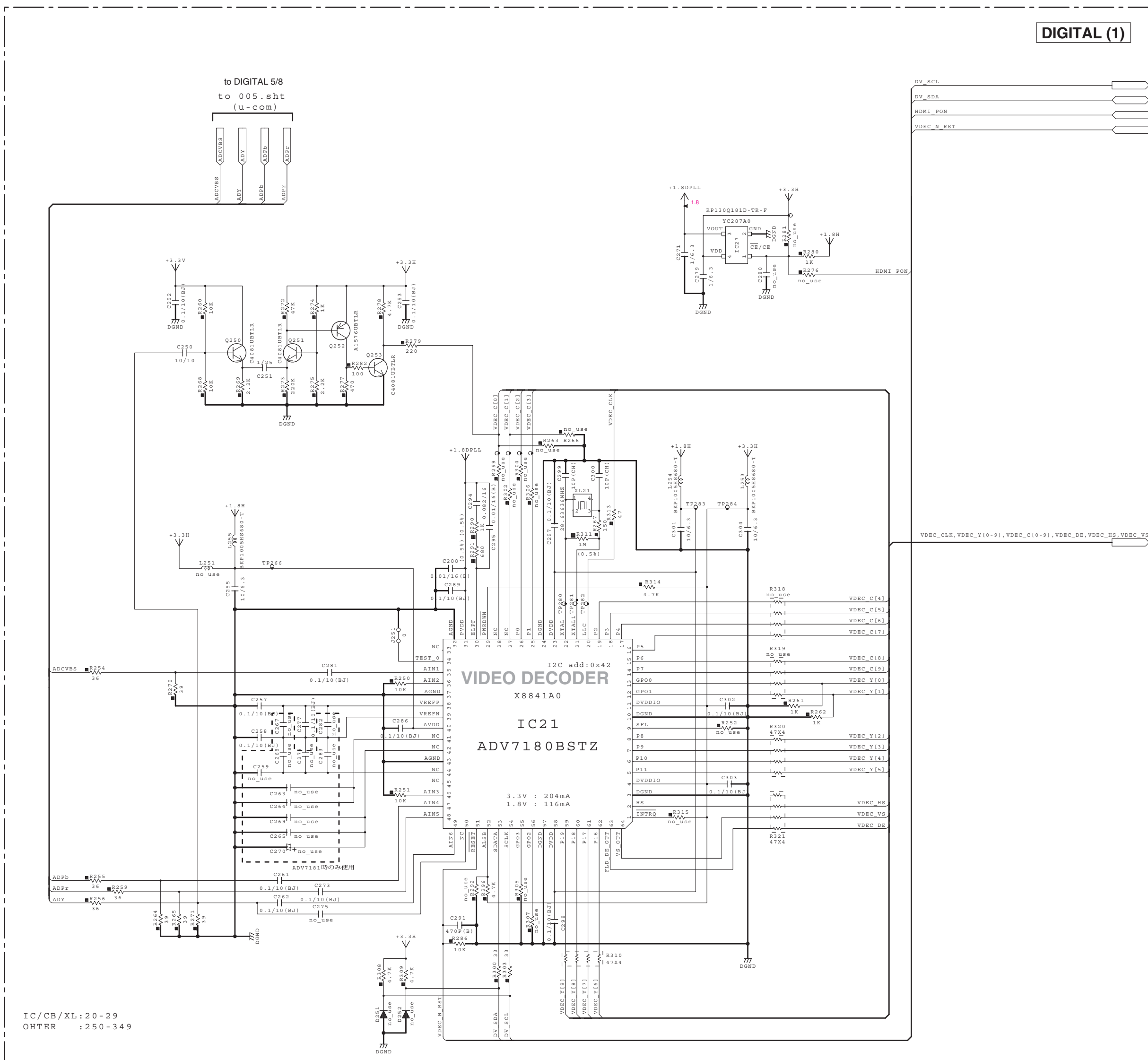
IC21: ADV7180BSTZ 10-bit, 4 x oversampling SDTV video decoder
