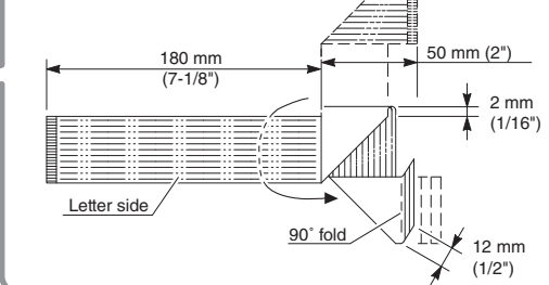
Flexible flat cable
