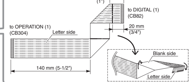
Flexible flat cable
