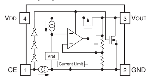
IC27: RP130Q181D-TR-F Voltage regulator
