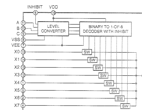
IC602 : HD74HC4051P Analog Multiplexers/Demultiplexers
