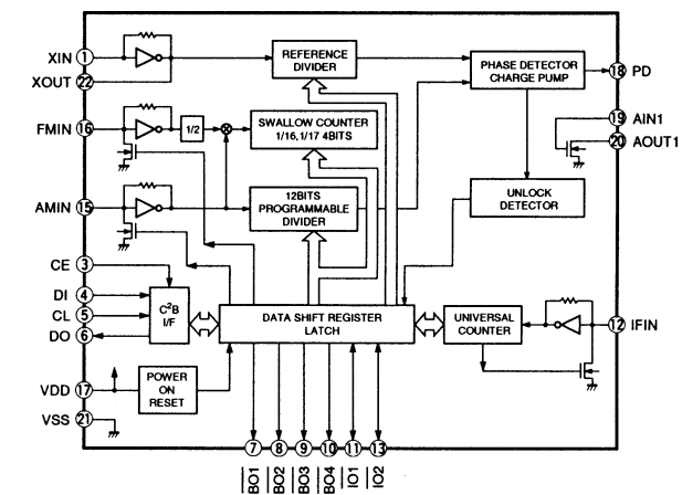
IC2 : LC72131 PLL Controller
