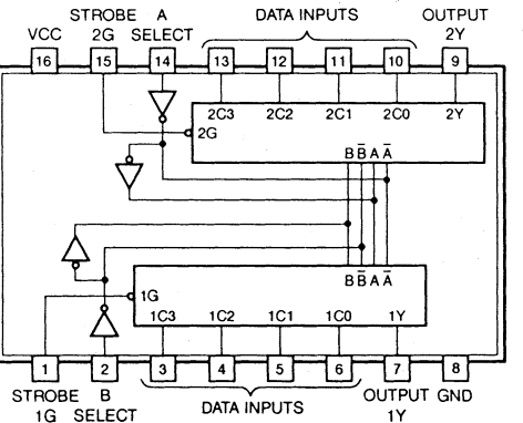
IC353 : HD74HC153P Dual 4 to 1 Data Selectors
