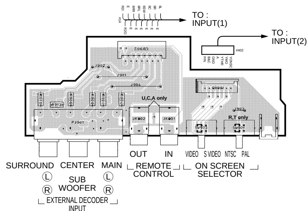
P.C.B. OPERATION (4)
