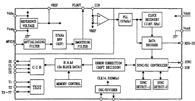
IC4 : LC72720N RDS Decoder & Controller
