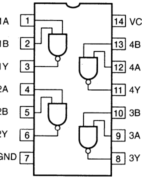
IC352 : HD74HC00P Quadruple 2-input Positive NAND Gates
