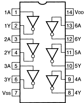
IC351 : TC74HC04AP Hex Inverters
