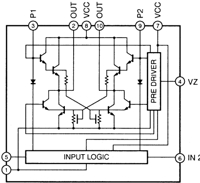
IC254 : LB1641 Motor Driver
