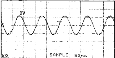
Point 6 (Pin13 of IC14) V : 2V/div H : 50 nsec/div DC range 1 : 1 probe
