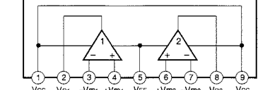
IC202 : \mu PC4570HA Dual OP-Amp
