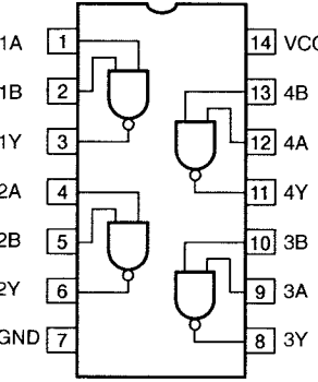
IC352 : HD74HC00P Quadruple 2-input Positive NAND Gates
