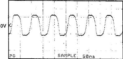
Point 5 (Pin13 of IC3) V : 2V/div H : 50 nsec/div DC range 1 : 1 probe
