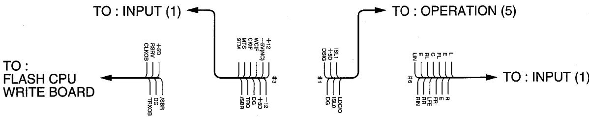
P.C.B. DSP Lead Type Device
