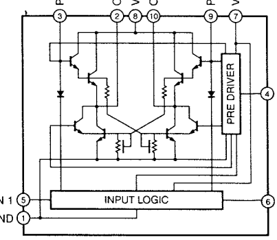
IC254 : LB1641 Motor Driver
