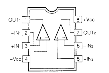
IC251~253, 257, 258 : \mu PC4570G2 Dual OP-Amp
