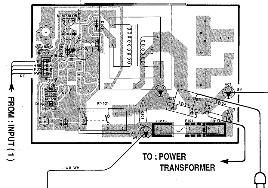
RX-V870 MAIN P. C. B. ( 3 )
