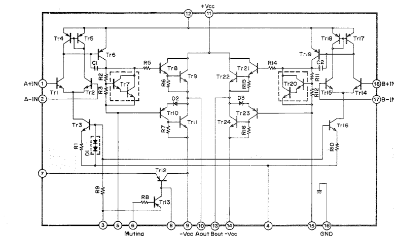
IC104 : STK4151V Power Amp
