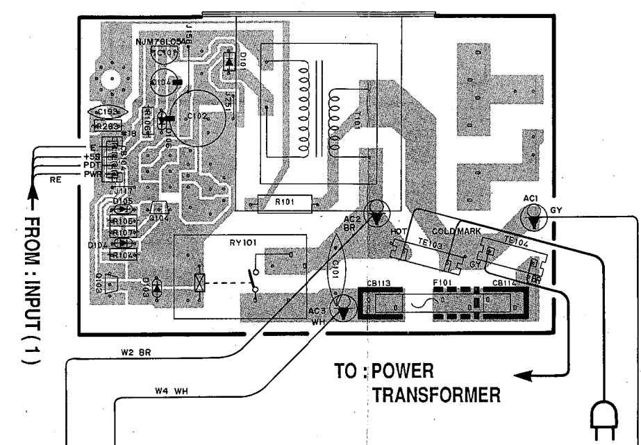
RX-V1070 MAIN P. C. B. ( 6 )
