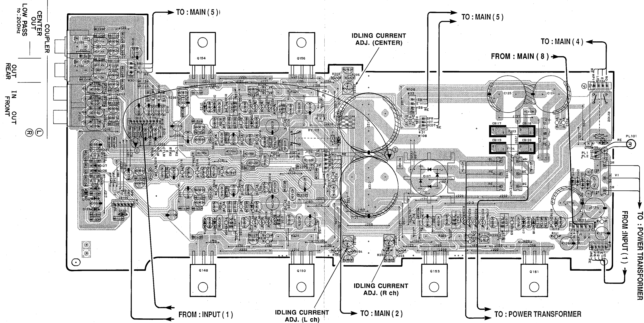
RX-V1070 MAIN P. C. B. ( 1 )
