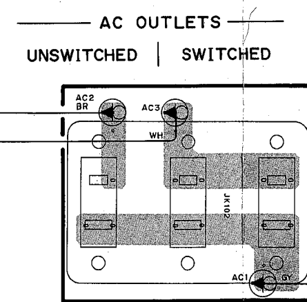
RX-V1070 MAIN P. C. B. ( 6 )
