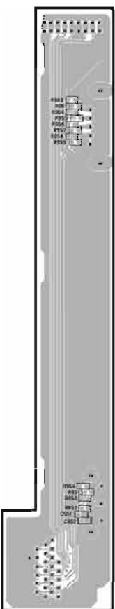
OPERATION (4) P.C.B.
