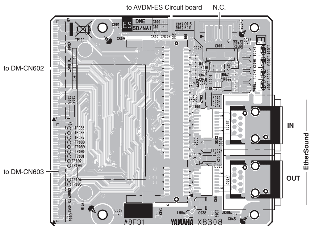
Component side (部品側)
