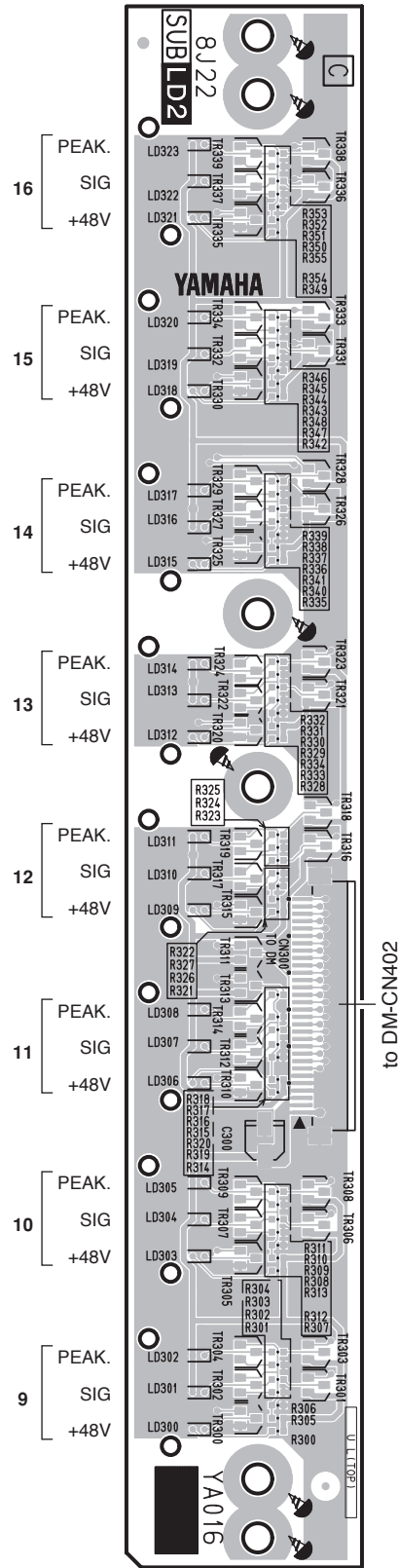
Component side (部品側)
