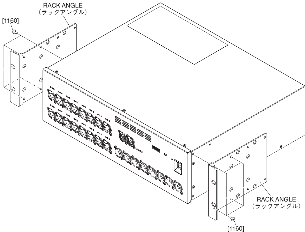
[1160]: BIND HEAD SCREW 4X8 (小ネジ+B I N D) 4.0X8 MFZN2B3 IT (WE99710R)
