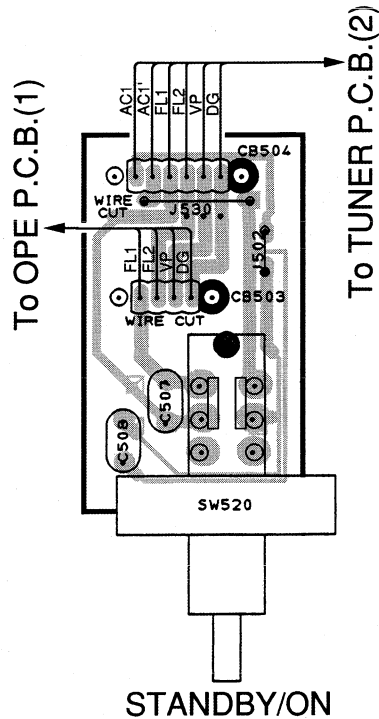
OPERATION P.C.B.(2)
