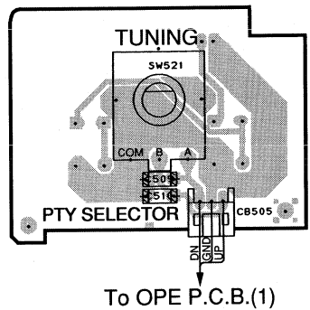
OPERATION P.C.B.(3)
