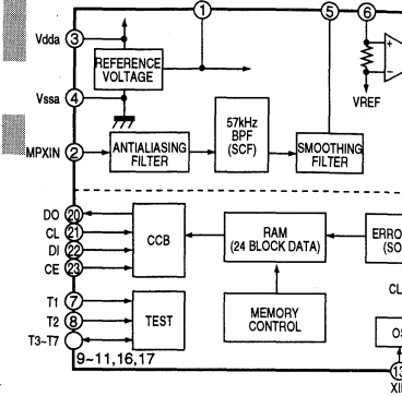
IC401 : LC72720N (RDS)
