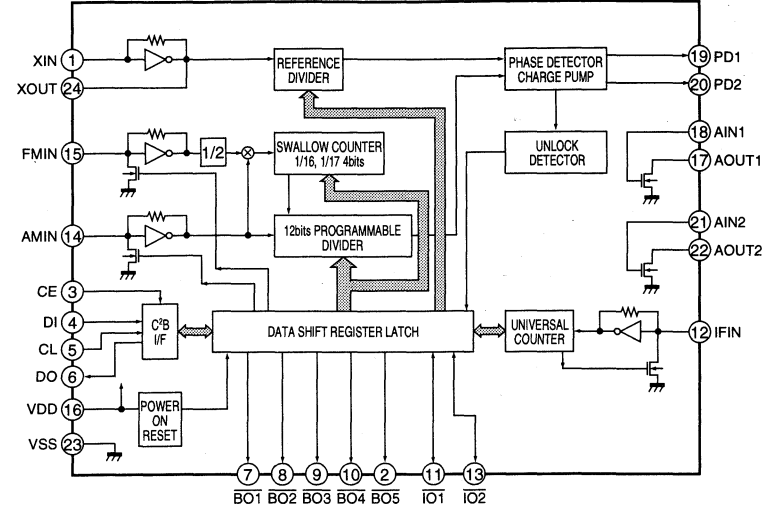
IC2 : LA1266 (AM/FM IF)
