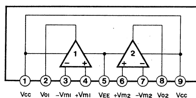
IC105: \mu PC4570HA (Dual Ope-amp)
