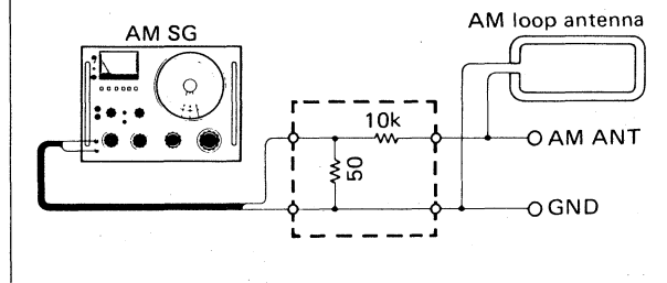
AM DUMMY ANTENNA CONNECTION
