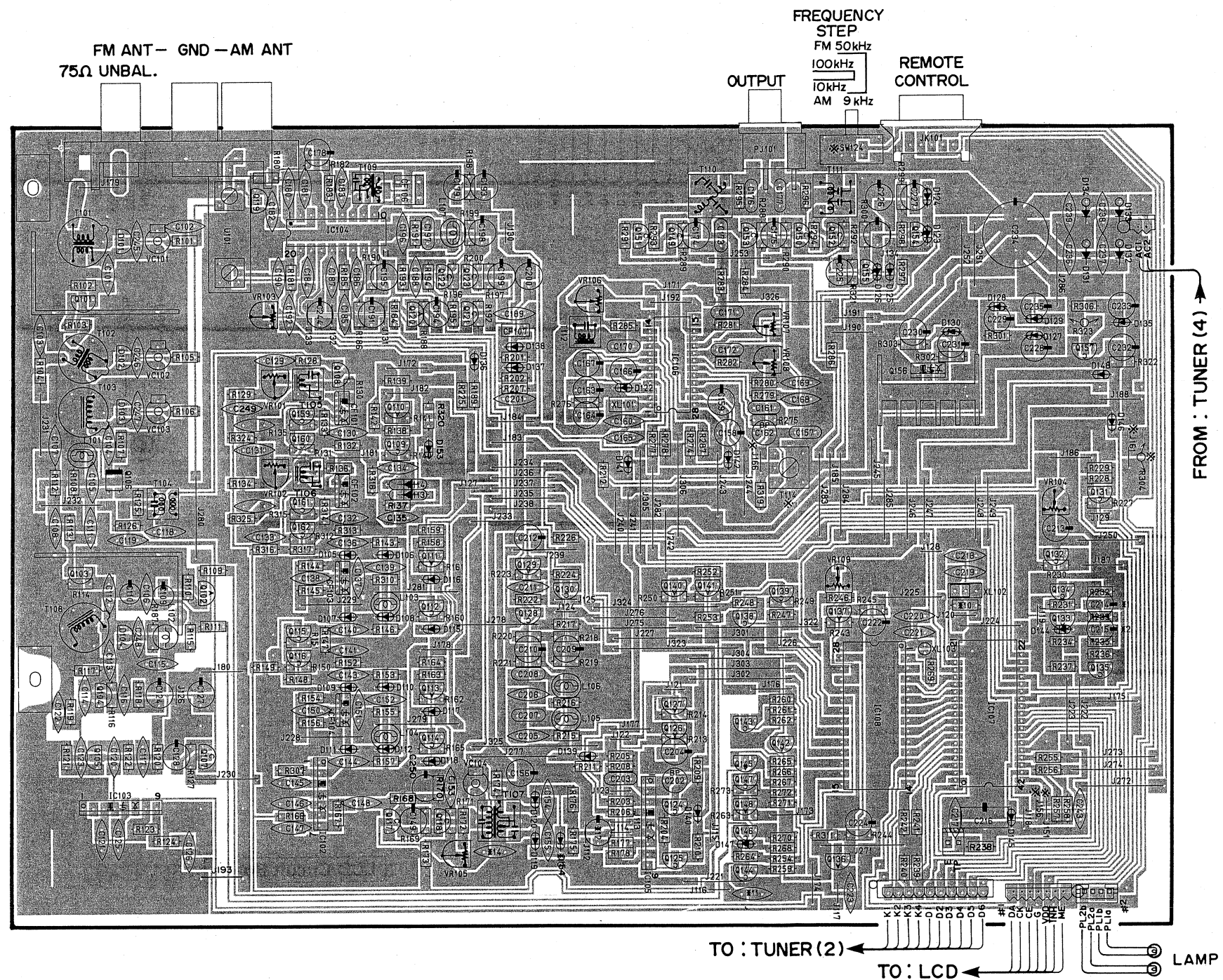
Tuner Circuit Board (1)
