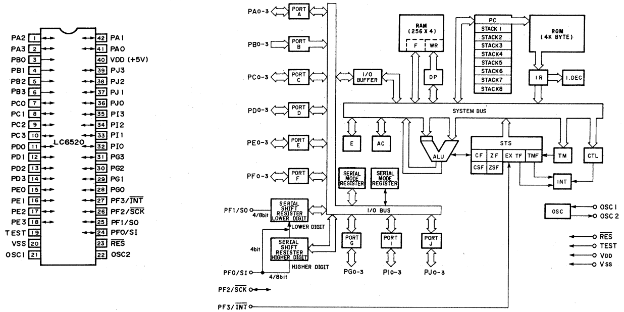
IC107: LC6520C-3235 (4-bit \mu -COM)
