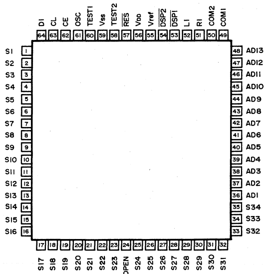
IC501: LC7583 (LCD Driver)
