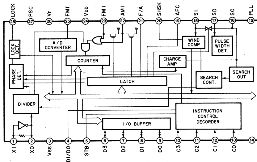
IC108: LC7210 (PLL)
