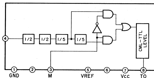
IC103: M54459L (Divider)
