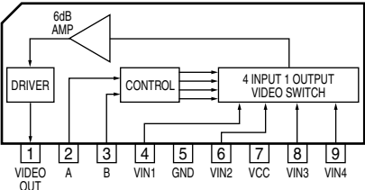
IC550 : LA7956 Video Switch
