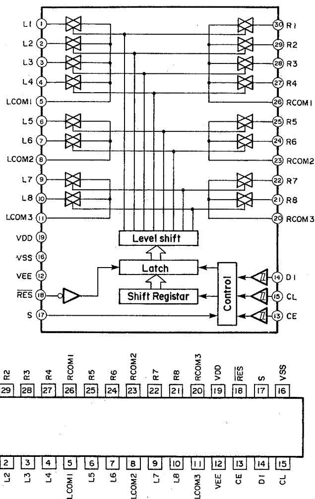
IC201 : LC7821N
