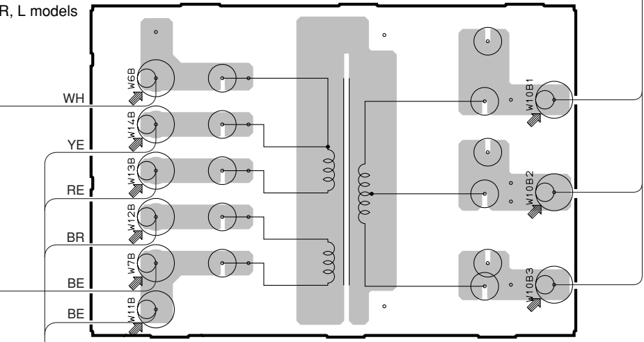
MAIN (8) P.C.B. (Side A)
