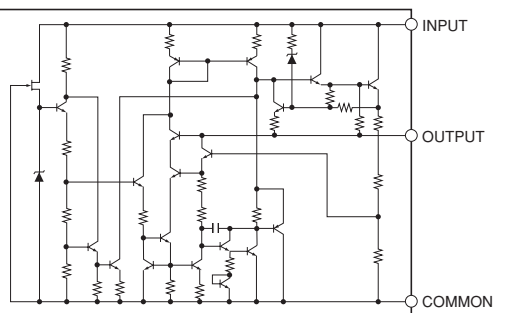
IC4: NJM78M15FA Voltage regulator
