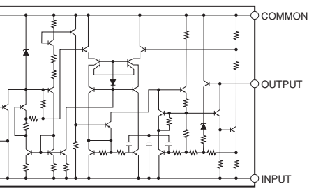
IC5: NJM79M15FA Voltage regulator
