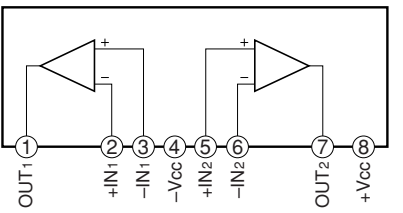
IC1, 2, 6: NJM4558L Dual operational amplifier
