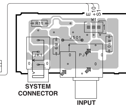
MAIN (4) P.C.B. (Side A)
