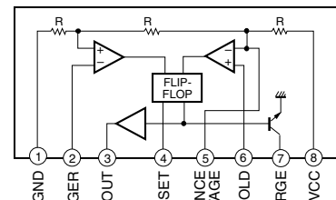
IC5: M51848L CR Timer
