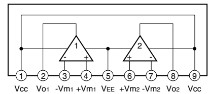
IC1, 4, 7-9: \mu PC4570HA Dual OP-Amp
