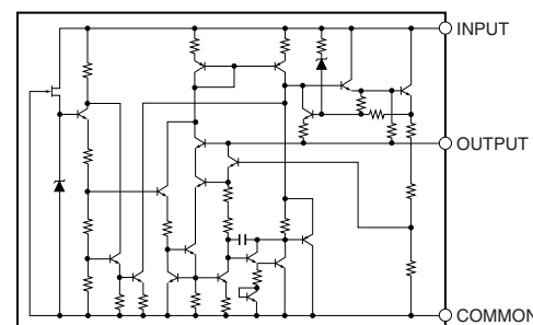
IC6: NJM78M12FA Voltage Regulator
