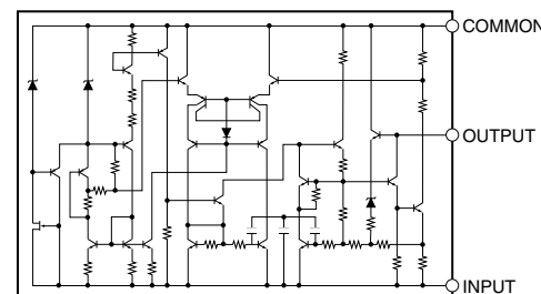
IC10: NJM79M12FA Voltage Regulator
