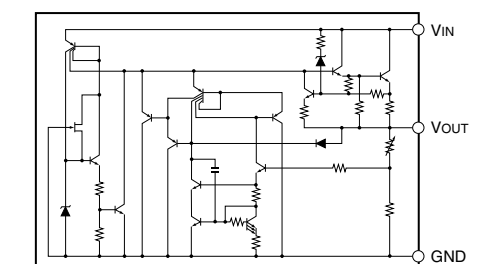
IC12: NJM78L08A Voltage Regulator
